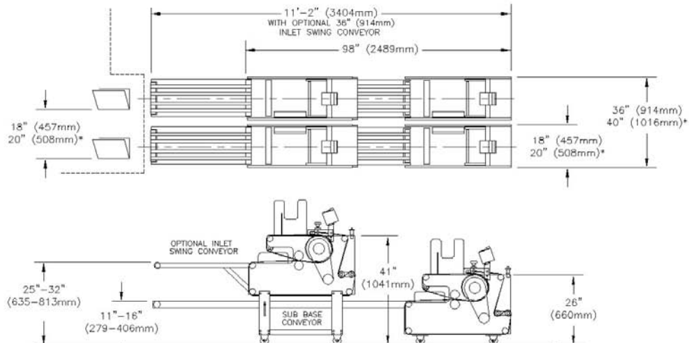
ELEVATION VIEW WITHOUT PIGGY-BACK CONVEYOR
